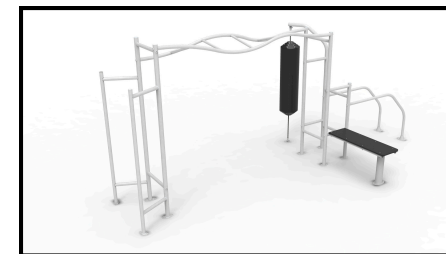
Satellite MIMAS
